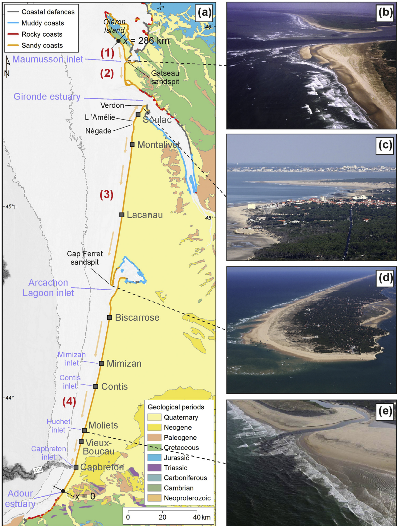
Fig. 1. Study area between x = 0 and x = 286 km essentially composed of sandy coasts with indication of the inherited geology. Note that rocks can locally outcrop in the intertidal and subtidal domain at some of the sandy beaches in the northern sector of Oléron and in south of the Gironde estuary (Chaumillon et al., 2008; Feniès et al., 2010). The grey squares indicate the location of the small coastal towns with their seafront more or less built on the coastal dunes. Four coastal compartments are distinguished with from north to south: (1) south Oléron coast; (2) Arvert peninsula; (3) Gironde coast; (4) Landes coast. The sandy arrows indicate the direction and magnitude of the net longshore drift. Aerial photographs of some relevant coastal forms: (b) the Maumusson inlet; (c) the coastal town of Soulac with the Gironde estuary in the background (Ph. J. Augereau, @Lacanau Council); (d) the Cap Ferret sandspit (@Observatoire de la Côte Aquitaine); (e) the wave-dominated Huchet inlet (Ph. I. Louvier).
