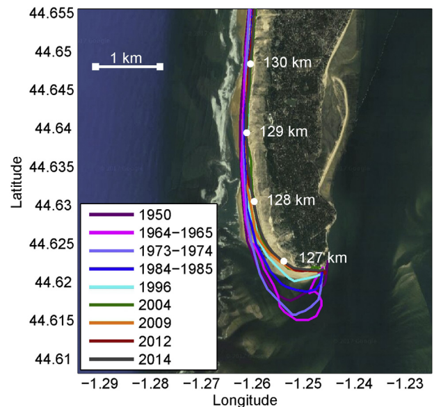
Fig. 10. Shoreline change between 1950 and 2014 at the Cap Ferret sandspit in the south of the Gironde coast.
