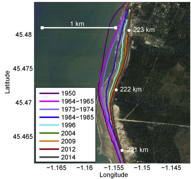
Fig. 9. Shoreline change between 1950 and 2014 along the Pointe de la Négade and Amélie in the north of the Gironde coast.
