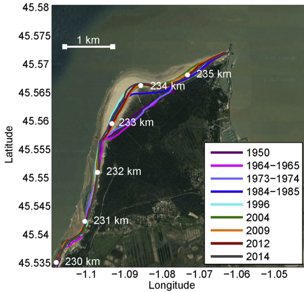
Fig. 8. Shoreline change between 1950 and 2014 along the coast south of the Gironde estuary.
