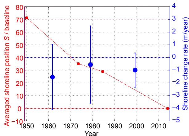
Fig. 11. Alongshore-averaged shoreline position S (red) and resulting erosion rate (blue) computed over the sectors (1), (2) and (3) indicated in Fig. 1. (For interpretation of the references to colour in this figure legend, the reader is referred to the web version of this article.)
