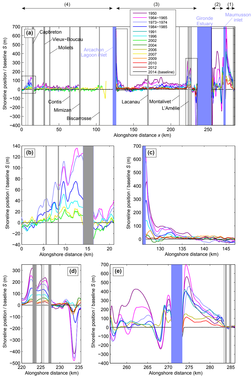
Fig. 5. (a) Time evolution of shoreline position S from south ( x = 0 ) to north ( y = 270 km) and from 1950 to 2014 with the dates coloured. Shoreline positions are all given with respect to the shoreline baseline defined in 2014, with positive S meaning that the shoreline is more seaward than in 2014. Coastal towns with hard defences as well as tidal inlets and estuaries interrupting the open coast are indicated by the vertical grey areas. Relevant coastal towns are also indicated. The four dashed black boxes indicate the zoomed areas provided in panels (b), (c), (d) and (e). (For interpretation of the references to colour in this figure legend, the reader is referred to the web version of this article.)
