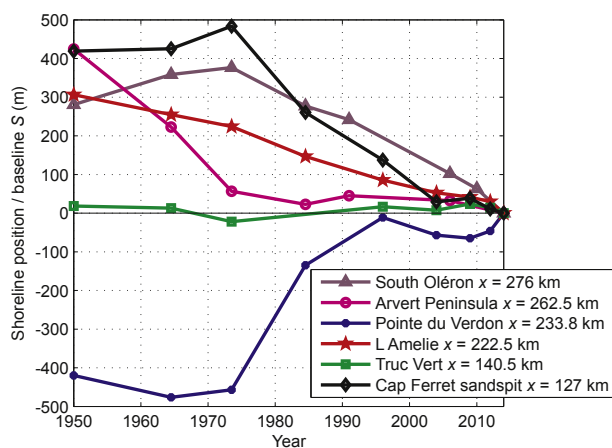
Fig. 6. Time evolution of shoreline position S at 6 representative locations in SW France. For all locations S = 0 is the shoreline position in 2014.
