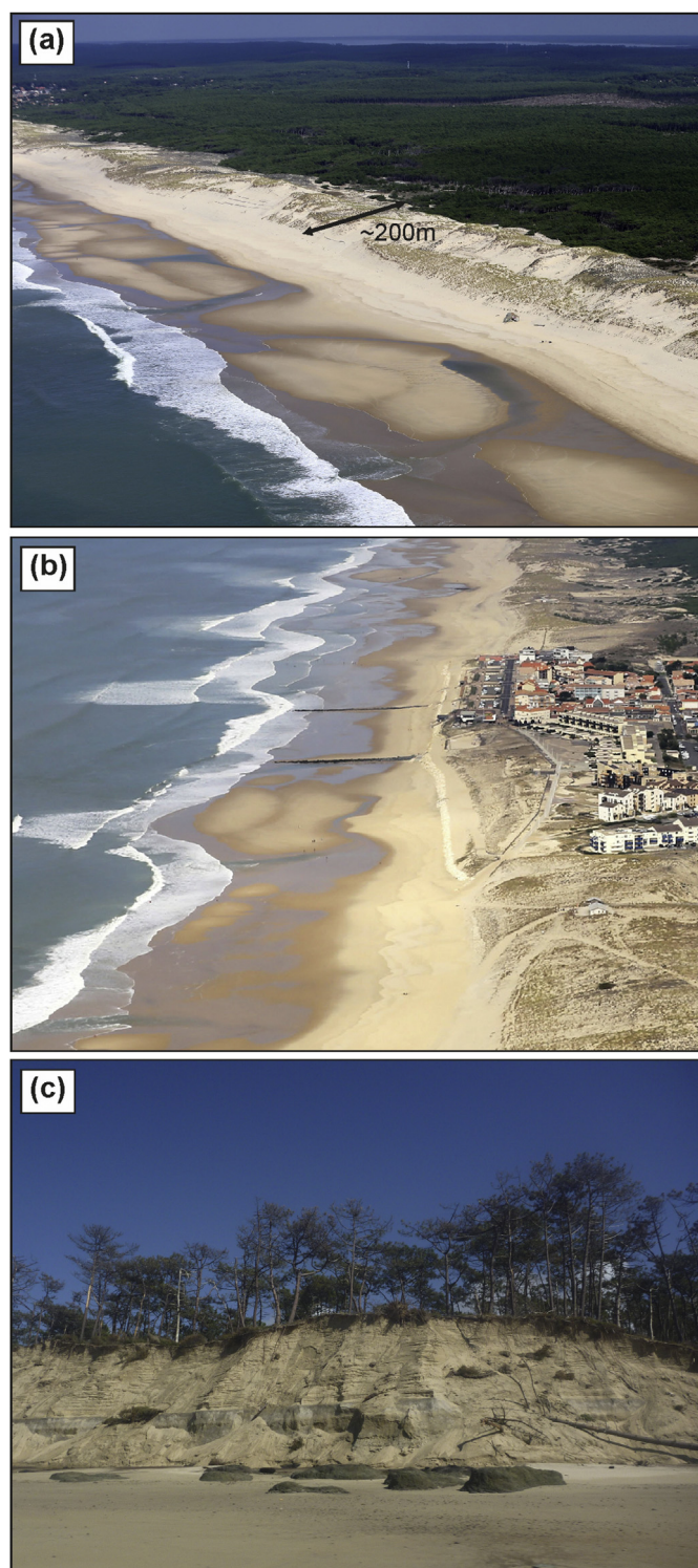
Fig. 2. Aerial photographs of (a) the typical landscape of the study area with sandy beaches backed by high and wide coastal dunes, (b) the coastal town of Lacanau with its seafront built on the dune, a similar setting to e.g. Montalivet and Mimizan and (c) localized areas under severe chronic erosion with the loss of the coastal dune exposing the coastal forest to marine erosion. Photographs (a,b) by J. Augereau (@Lacanau Council) and (c) by B. Castelle.
